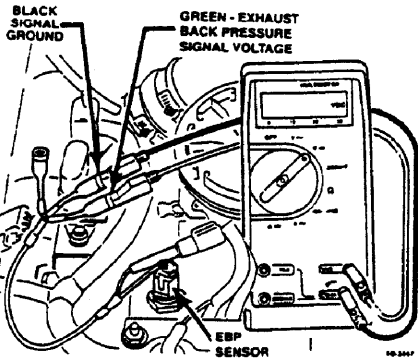
EXHAUST BACK PRESSURE
